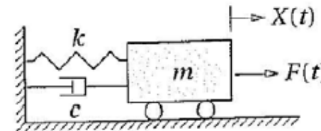
Figure 4.17 SDOF system subjected to random load F(t) .
