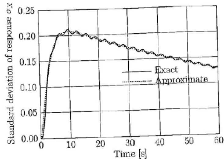
Figure 4.14 Transient standard deviation of the displacement response.
