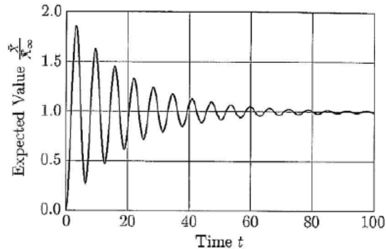
Figure 4.7 Expected displacement response for SDOF systems.
