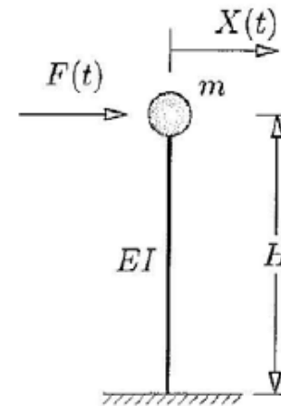
Figure 4.8 Cantilever structure subjected to lateral loading.
