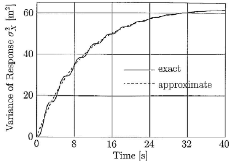
Figure 4.11 Variance of response to white noise excitation.
