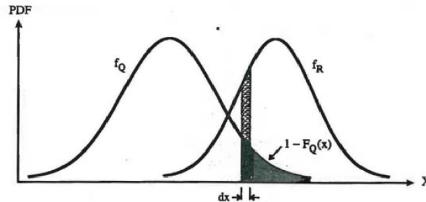
PDFs of load ( Q ) and resistance ( R ).
