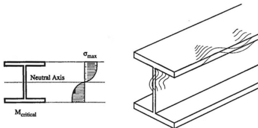
Local buckling in a steel beam.
